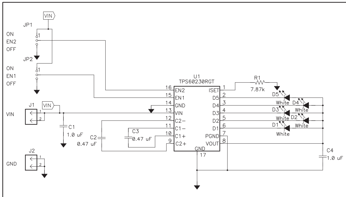
Figure 5. TPS60230EVM-047 Schematic
